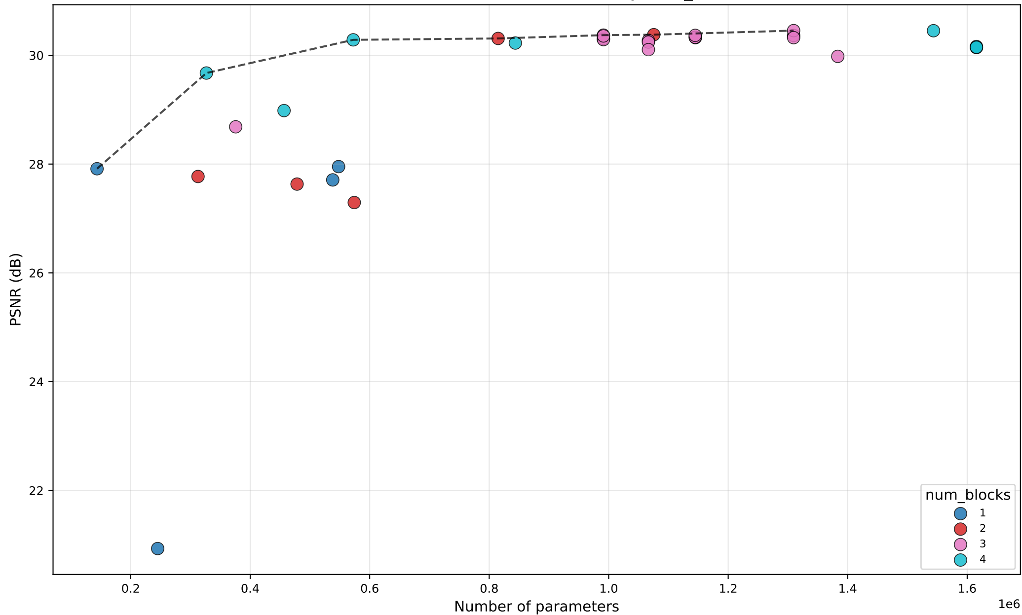
PSNR vs #Params — SRFormer — by num_blocks
